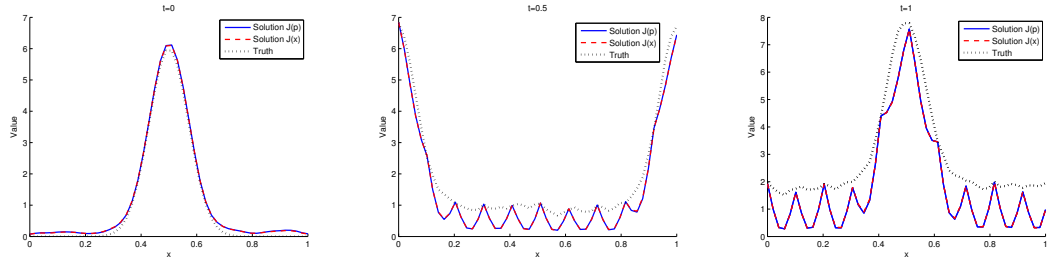
Figure 4.8: Assimilation window time series left to right, t = 0 , t = n/2 and t = n . Truth (black-dashed line), wc4DVAR \mathcal{J}(\mathbf{x}) solution (red line), wc4DVAR \mathcal{J}(\mathbf{p}) solution (blue line).
