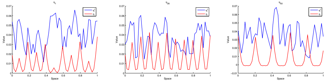
Figure 4.9: Model error time series left to right, t = 0 , t = n/2 and t = n . Estimated model error (red line) using wc4DVAR \mathcal{J}(\mathbf{p}) . True model error (blue line).
