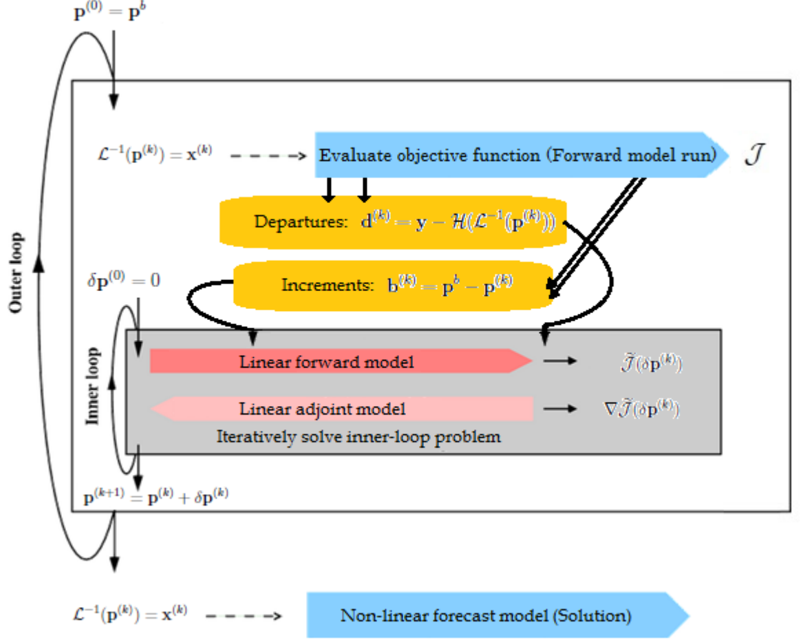
Figure 2.3: Illustration of Weak-Constraint Incremental 4DVAR, \delta \mathbf{p} formulation. (Diagram template courtesy of ECMWF presentation by Sebastien Lafont)
