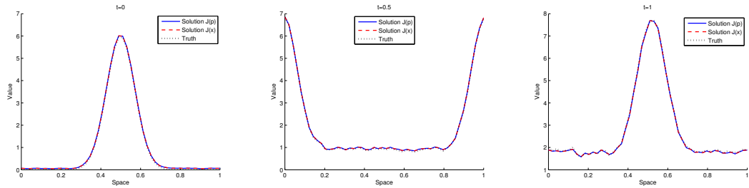
Figure 4.5: Assimilation window time series left to right, t = 0 , t = n/2 and t = n . Truth (black-dashed line), wc4DVAR \mathcal{J}(\mathbf{x}) solution (red line), wc4DVAR \mathcal{J}(\mathbf{p}) solution (blue line).
