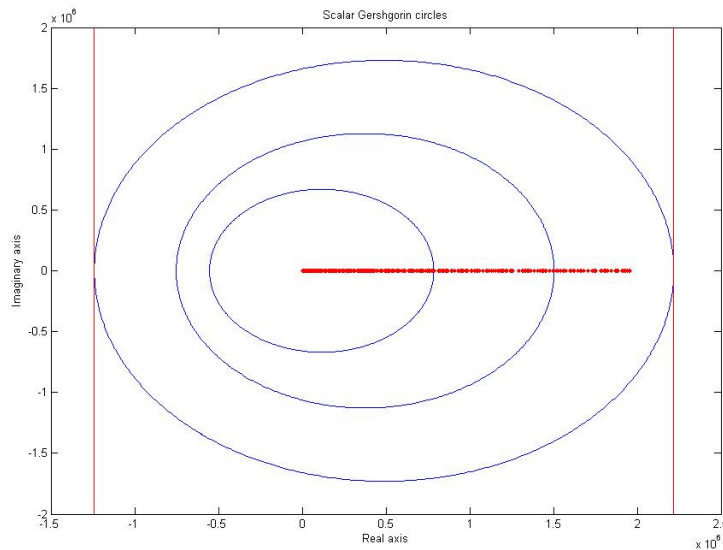
Figure 6.2: Scalar Geršgorin theorem applied to \mathbf{S}_x where \kappa(\mathbf{S}_x) = 3.912 \times 10^6 . Eigenvalues of \mathbf{S}_x (small red circles). Geršgorin discs (large blue circles) and estimated upper and lower bounds of the scalar Geršgorin Theorem (red vertical lines).
